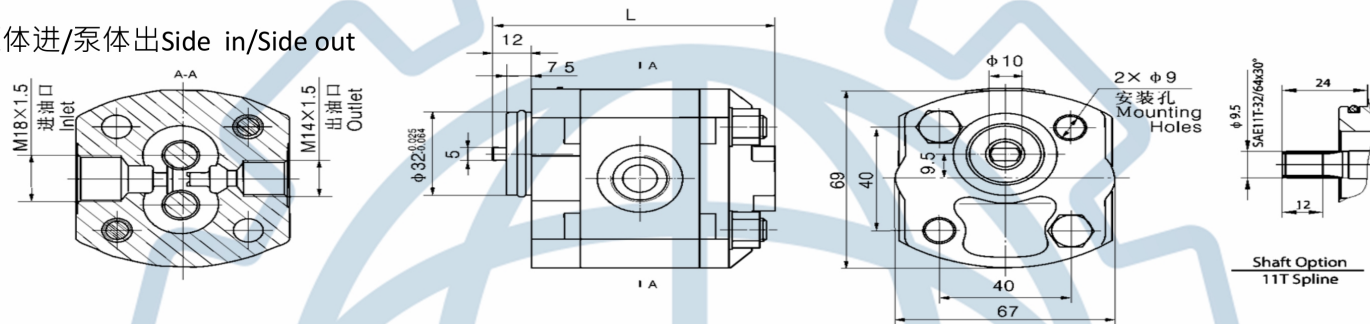
后盖进/后盖出 Rear in/Rear out
