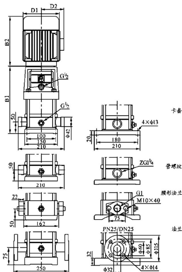
外形尺寸图 Overall and Dimensions Figure
