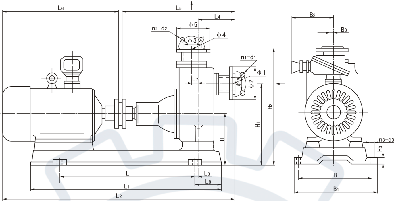
外形尺寸图 Overall and Dimensions Figure
